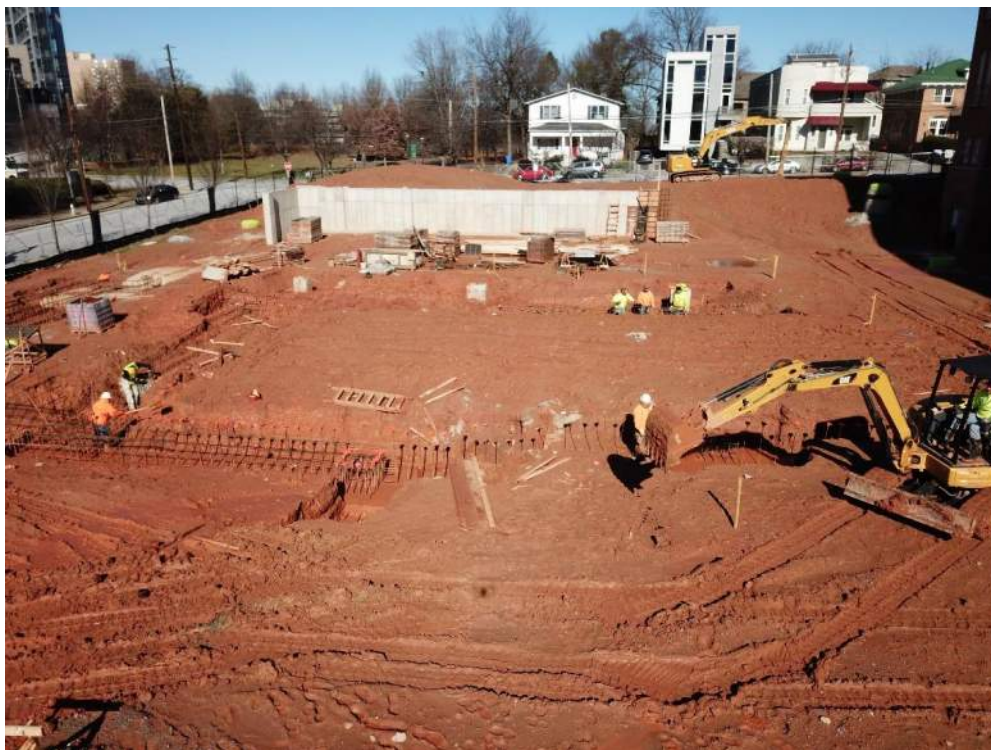
Aerial view of Area 1 concrete footers and retaining wall facing North
