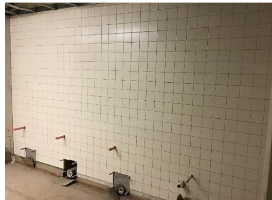
Wall Tile Installation at 2 nd Floor Restroom
