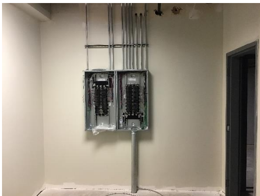
Electrical Panelboard Installed
