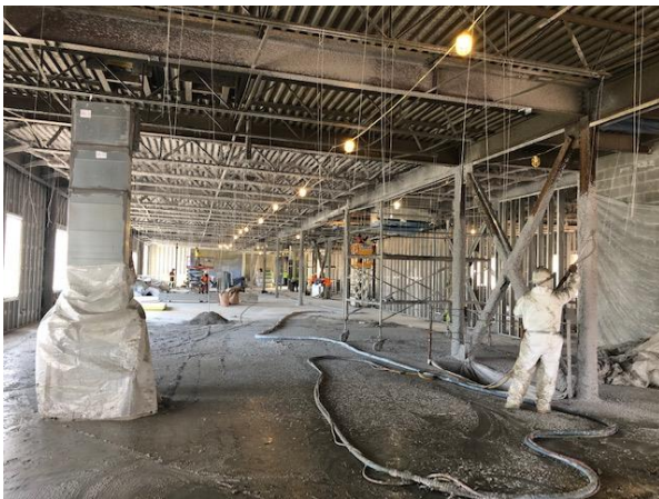
Fireproofing 3 rd floor WPA
