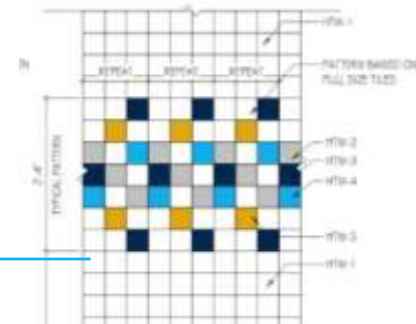
UNISEX RESTROOM WALL TILE
