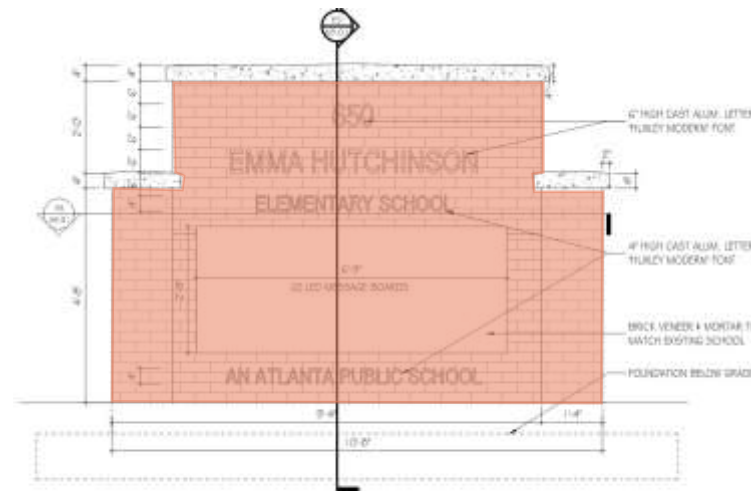
MONUMENT SIGN
