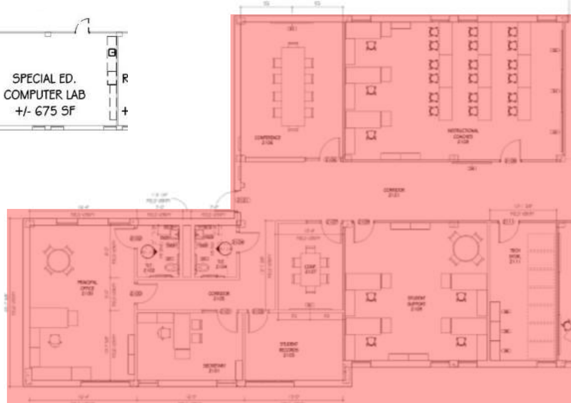
NEW ADMINISTRATIVE SUITE LAYOUT
