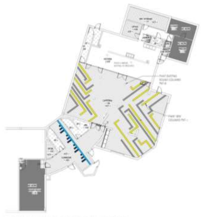
FLOOR PATTERN PLAN – BASEMENT LEVEL
