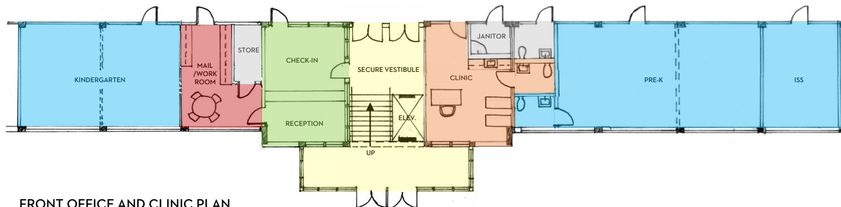
FRONT OFFICE AND CLINIC PLAN
